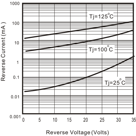
Fig.1 - Reverse Characteristics
