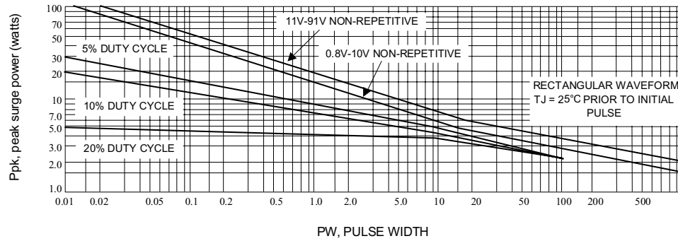
Fig. 5-MAXIMUM SURGE POWER
