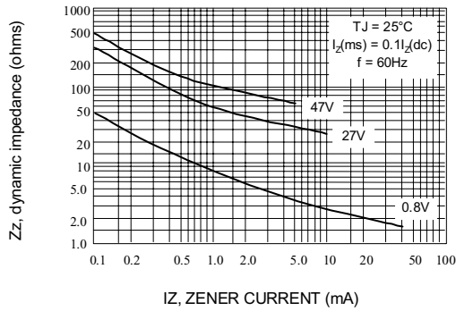
Fig. 6-EFFECT OF ZENER CURRENT ON ZENER IMPEDANCE
