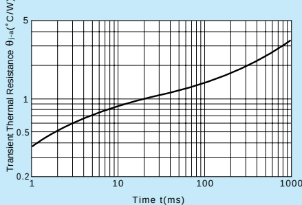
\theta_{JA}-t Characteristics
