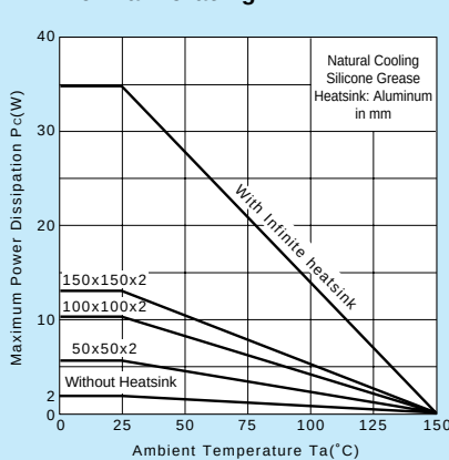
P_C-Ta Derating
