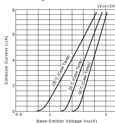
I C -V BE Temperature Characteristics (Typical)
