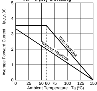
Ta—IF(AV) Derating
