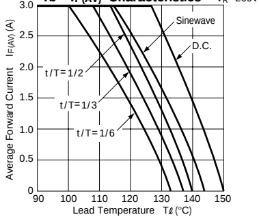
Tl—IF(AV) Characteristics
