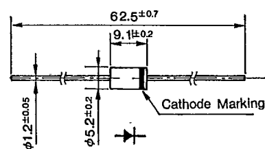
Outline Drawing ④
