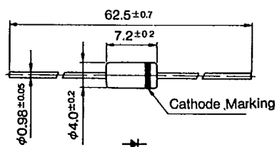
Outline Drawing ②
