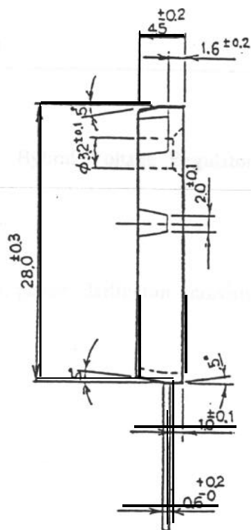
Fig-1 Outline Drawings, Dimensions and Pin Connections [Sanken lead forming LF500]
