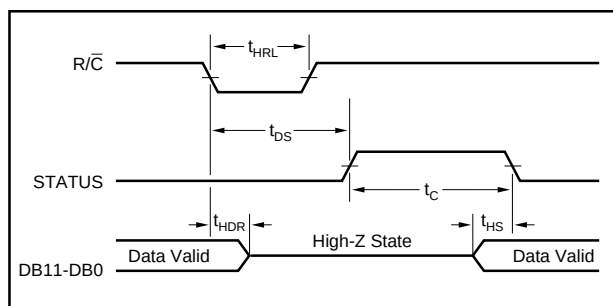
FIGURE 1. R/\bar{C} Pulse Low—Outputs Enabled After Conversions.
