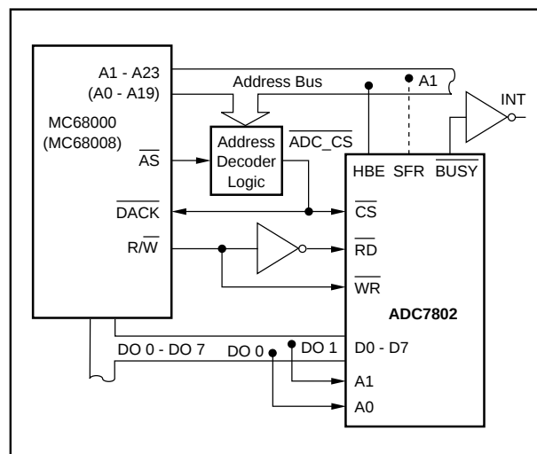
FIGURE 14. Interface to Motorola Microprocessors.
