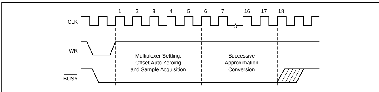
FIGURE 2. Converter Timing.
