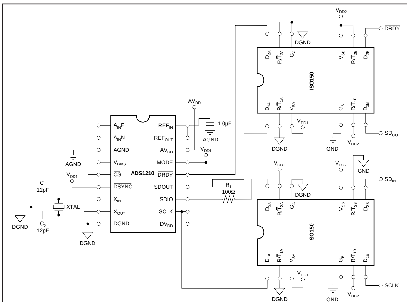
FIGURE 33. Isolated Four-Wire Interface.
