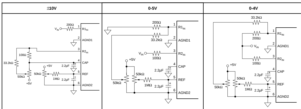
FIGURE 7a. Circuit Diagrams (With Hardware Trim).
