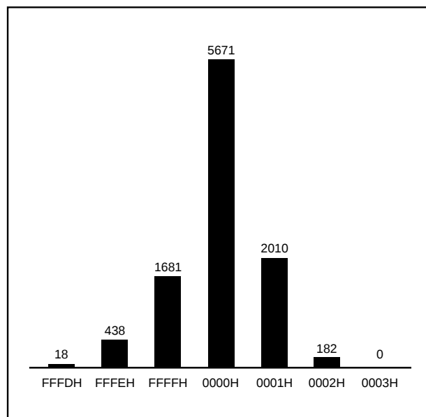
FIGURE 13. Histogram of 10,000 Conversions with Input Grounded.
