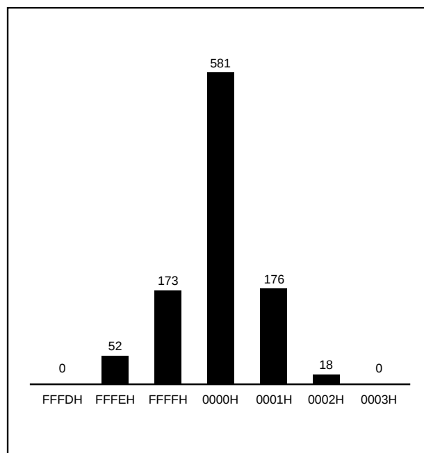
FIGURE 12. Histogram of 1000 Conversions with Input Grounded.
