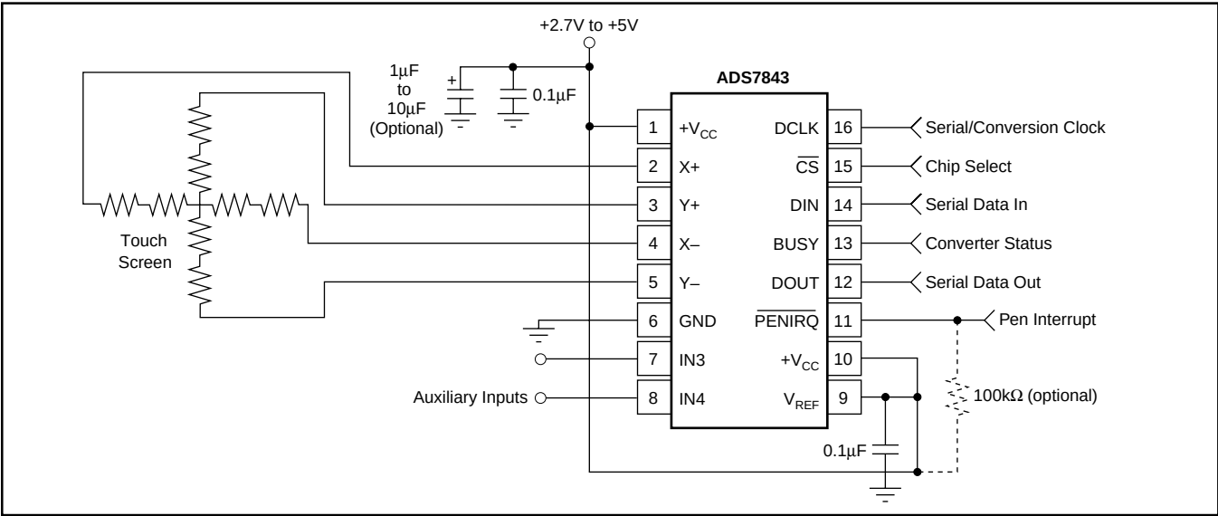
FIGURE 1. Basic Operation of the ADS7843.
