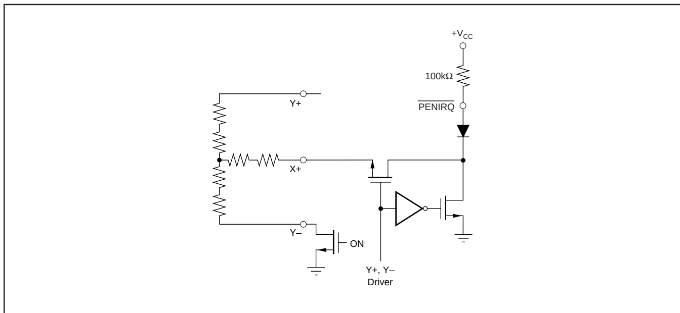
FIGURE 15. PENIROQ Functional Block Diagram.
