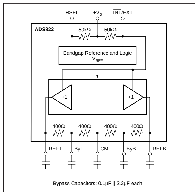
FIGURE 6. Equivalent Reference Circuit with Recommended Reference Bypassing.
