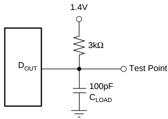
Load Circuit for t_{dO} , t_r , and t_f
