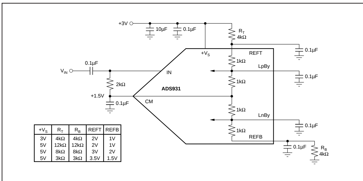
FIGURE 6. Low-cost Solution to Supply External Reference Voltages.
