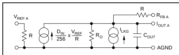
FIGURE 2. Simplified Circuit Diagram for DAC A.
