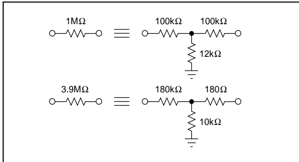
FIGURE 6. Equivalent Resistances.
