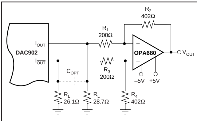
FIGURE 4. Difference Amplifier Provides Differential to Single-Ended Conversion and AC-Coupling.
