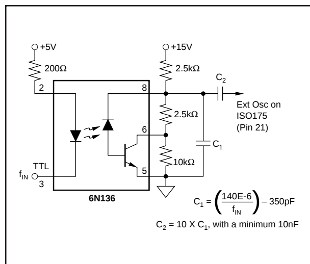
FIGURE 3. Synchronization with Isolated Drive Circuit for Ext Osc Pin.
