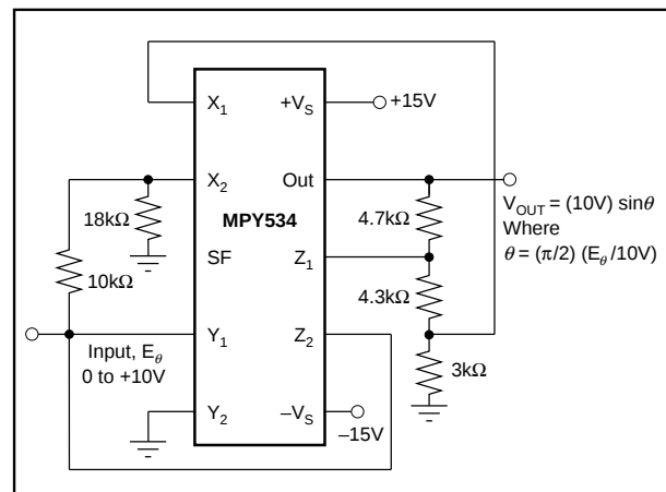
FIGURE 8. Sine-Function Generator.
