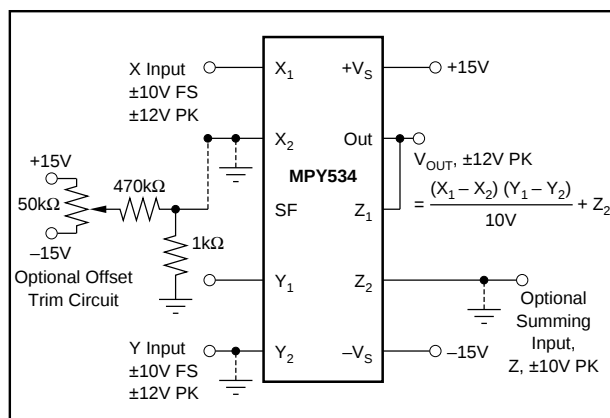
FIGURE 1. Basic Multiplier Connection.
