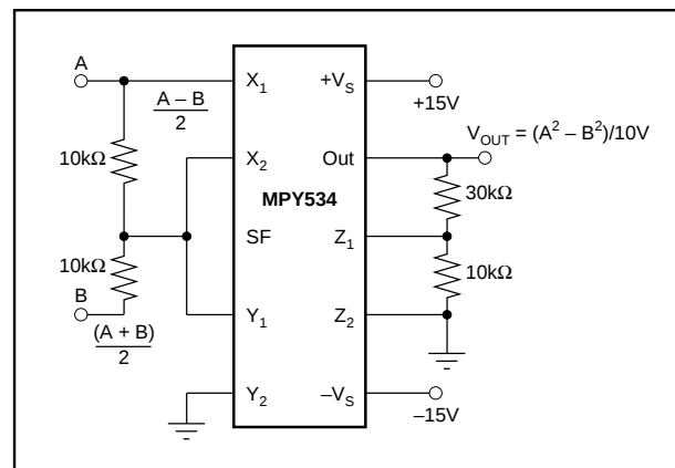
FIGURE 6. Difference-of-Squares.
