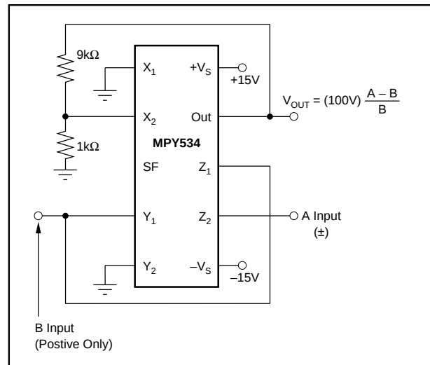
FIGURE 10. Percentage Computer.
