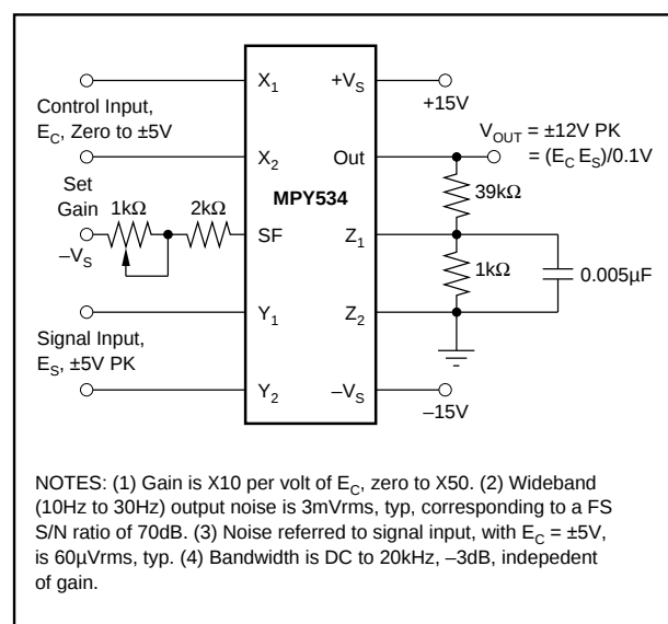
FIGURE 7. Voltage-Controlled Amplifier.
