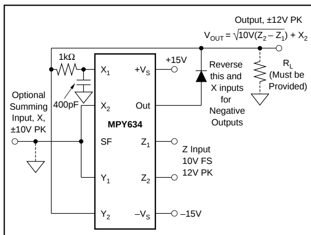
FIGURE 5. Square-Rooter Connection.
