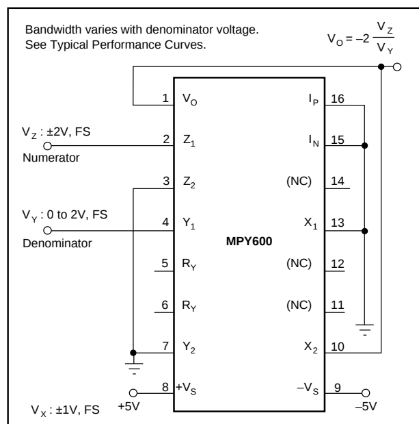
FIGURE 7. Divider Circuit.
