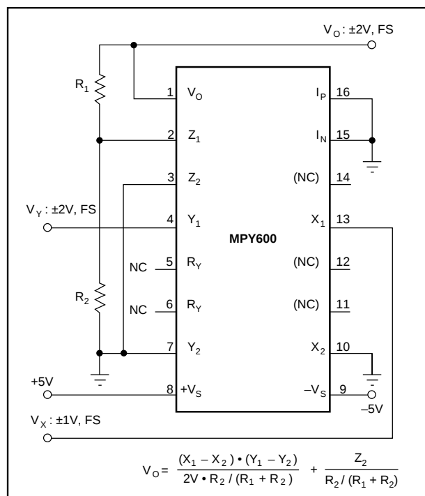
FIGURE 2. Adjusting the Scale Factor with Feedback.
