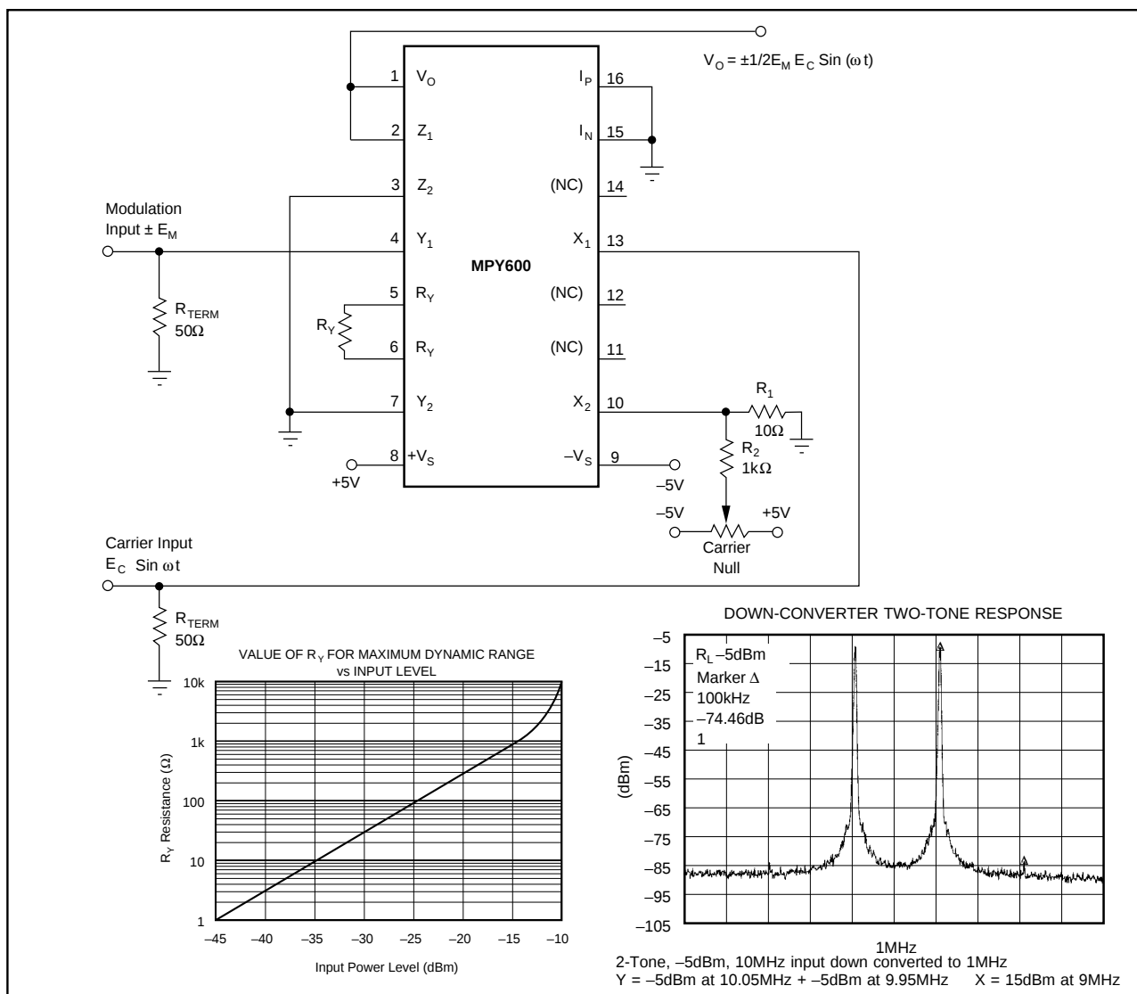
FIGURE 5. Balanced Modulator.
