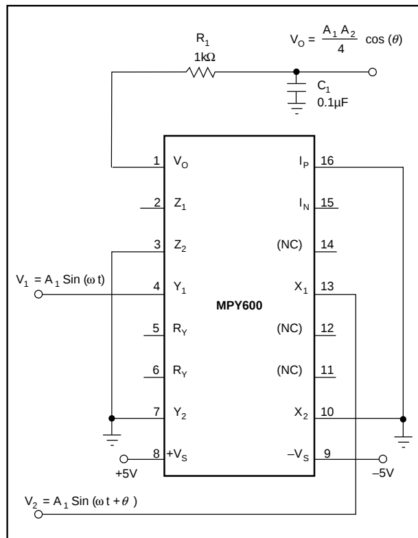
FIGURE 10. Phase Detector.
