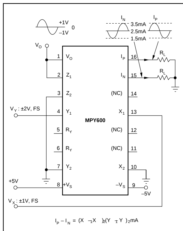
FIGURE 3. Current Output Connection.
