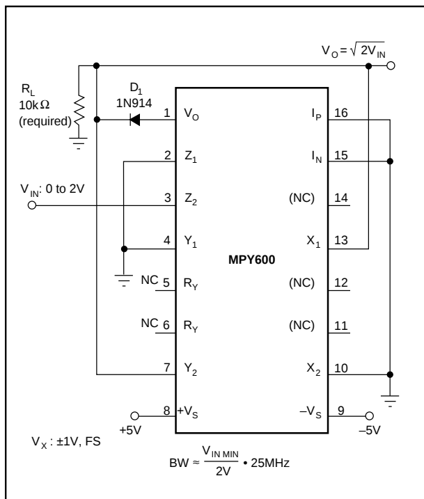
FIGURE 8. Square-Root Circuit.
