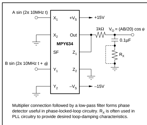
FIGURE 6. Phase Detector.
