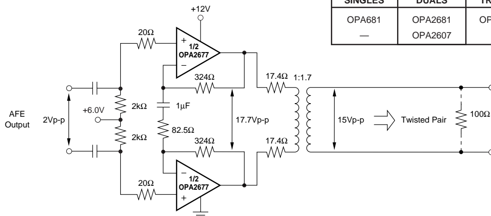
Single Supply ADSL Upstream Driver
