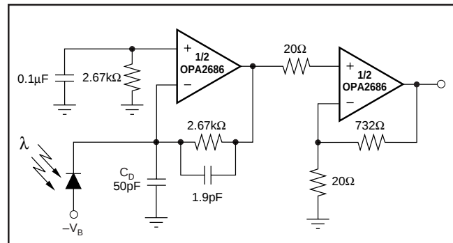
FIGURE 4. High Gain, Wideband Transimpedance Amplifier.
