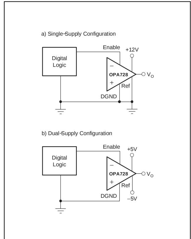
Figure 1. Enable Reference Pin Connection for Single- and Dual-Supply Configurations
