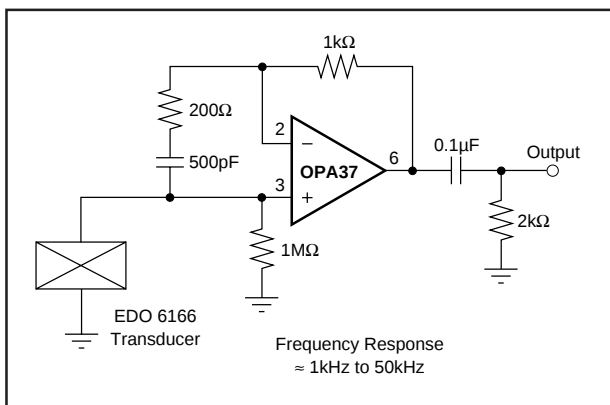
FIGURE 13. Hydrophone Preamplifier.
