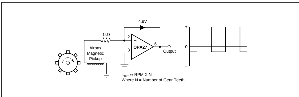
FIGURE 21. Magnetic Tachometer.
