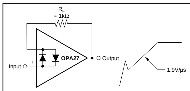
FIGURE 6. Pulsed Operation.
