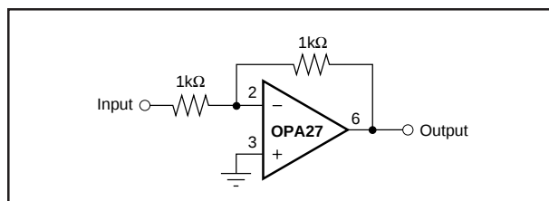
FIGURE 8. Unity-Gain Inverting Amplifier.
