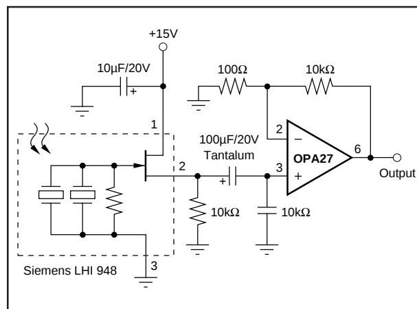
FIGURE 20. Balanced Pyroelectric Infrared Detector.
