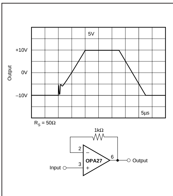
FIGURE 17. Unity-Gain Buffer.
