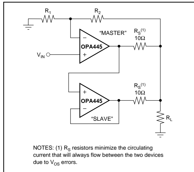
FIGURE 7. Parallel Amplifiers Increase Output Current Capability.
