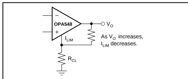
FIGURE 20. Single Quadrant V \cdot I Limiting.
