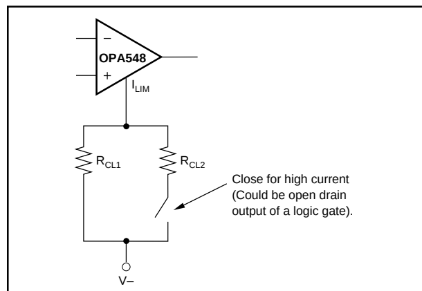
FIGURE 19. Multiple Current Limit Values.
