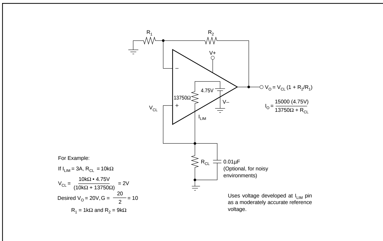
FIGURE 15. Voltage Source.
