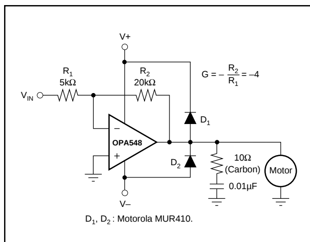
FIGURE 14. Motor Drive Circuit.
