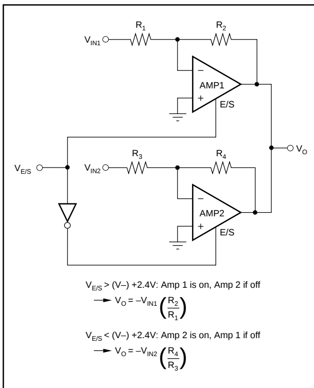
FIGURE 18. Switched Amplifier.
