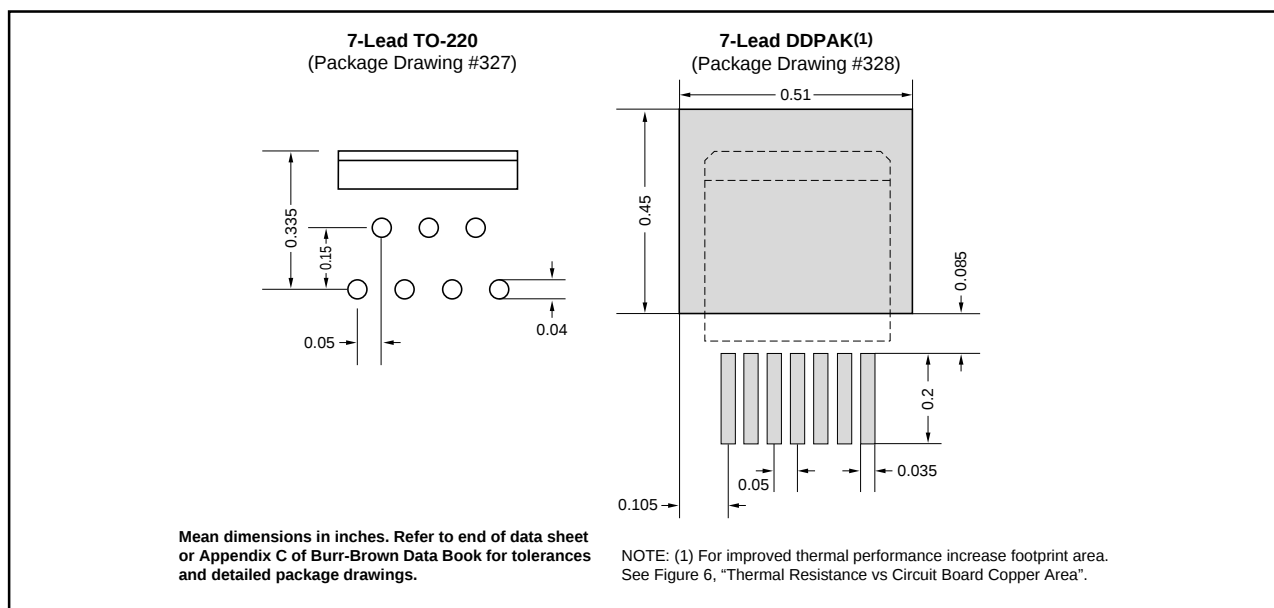
FIGURE 4. TO-220 and DDPAK Solder Footprints.
