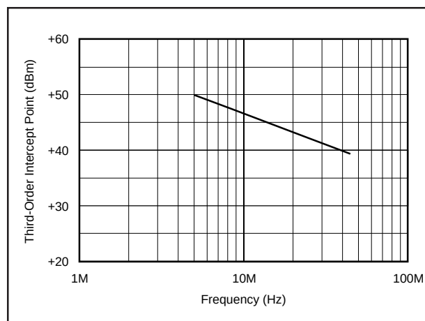
FIGURE 7. Single-Tone, 3rd-Order Intercept Point vs Frequency.
