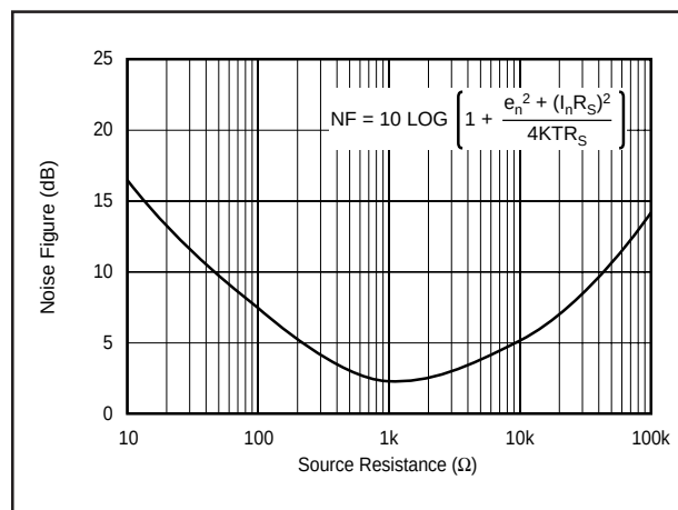
FIGURE 8. Noise Figure vs Source Resistance.
