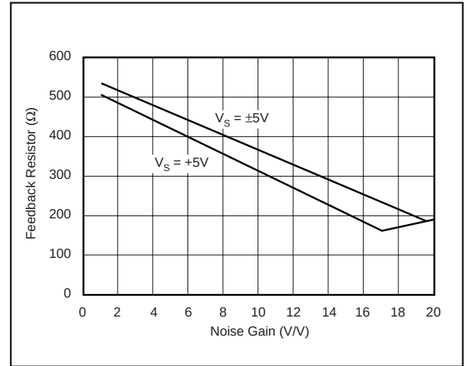
FIGURE 15. Recommended Feedback Resistor vs Noise Gain.
