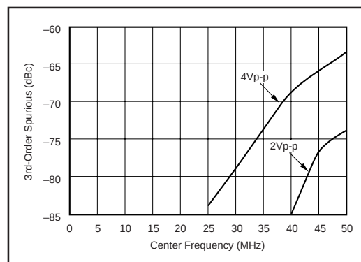
Measured 2-Tone, 3rd-Order Distortion for Differential ADC Driver.
