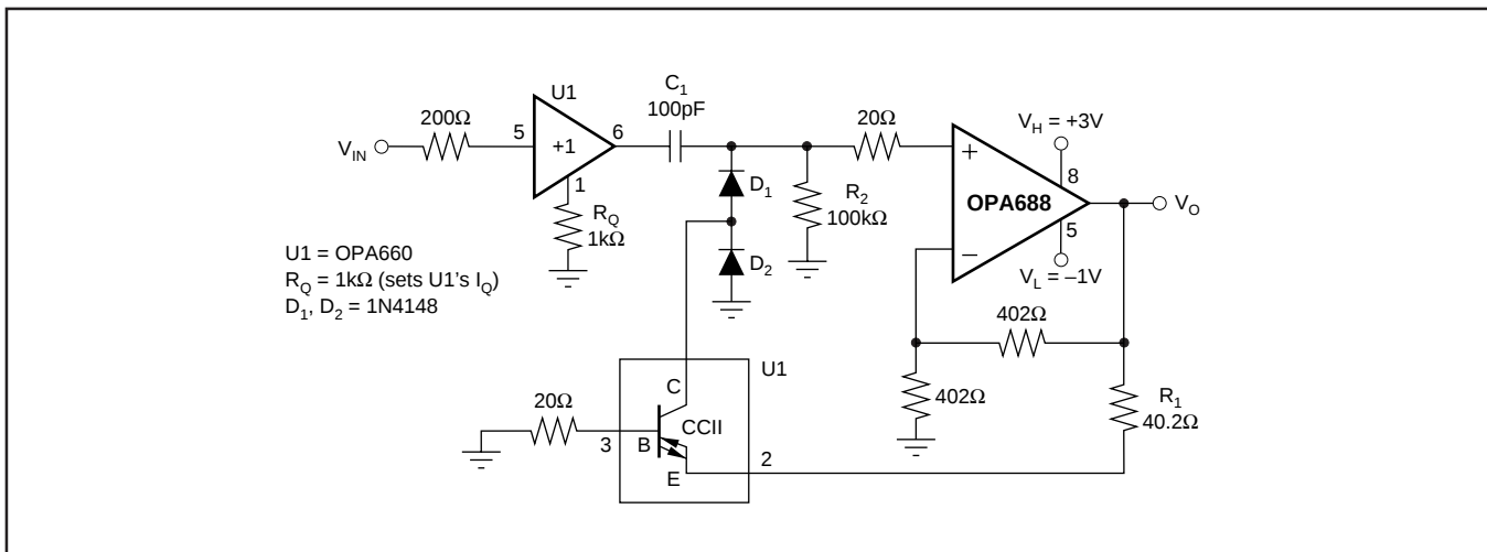
FIGURE 7. DC Restorer.
