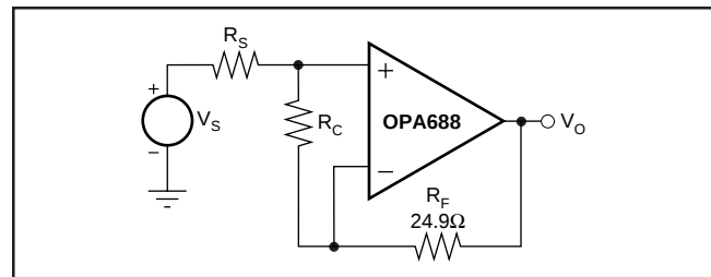
FIGURE 6. Unity-Gain Buffer.
