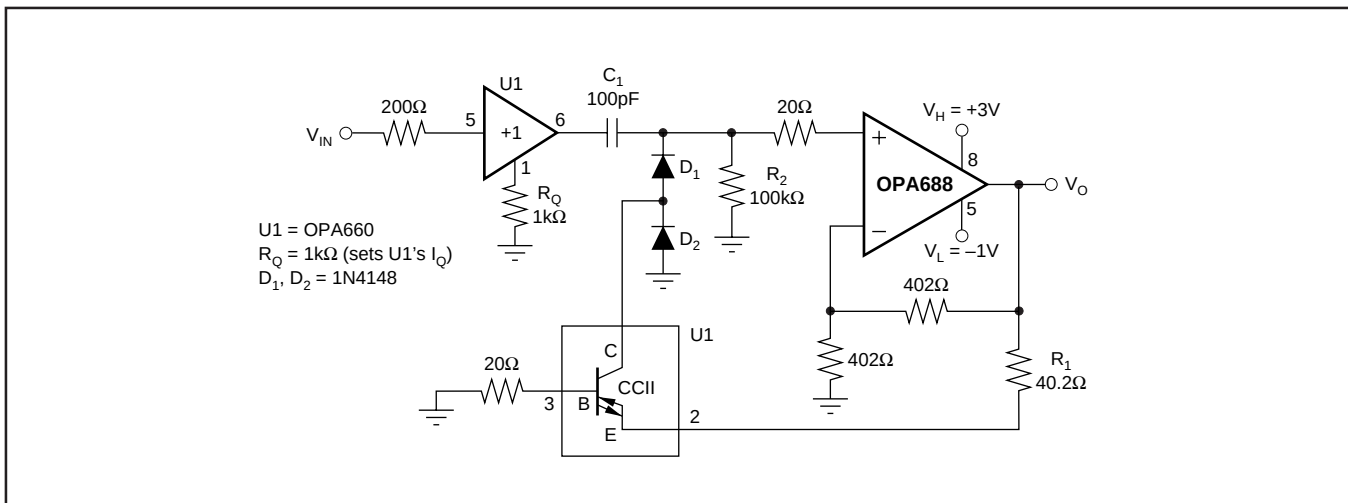
FIGURE 7. DC Restorer.
