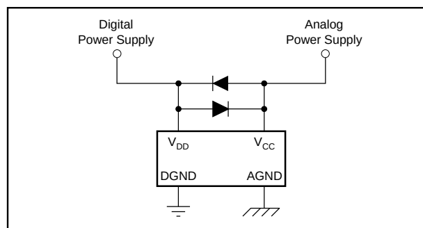
FIGURE 9. Latch-up Prevention Circuit.
