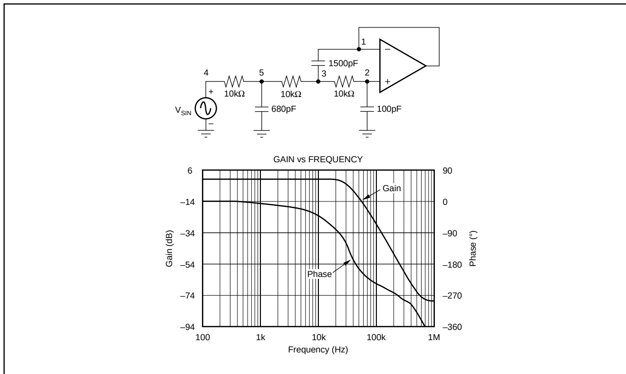
FIGURE 14. 3rd-Order LPF.
