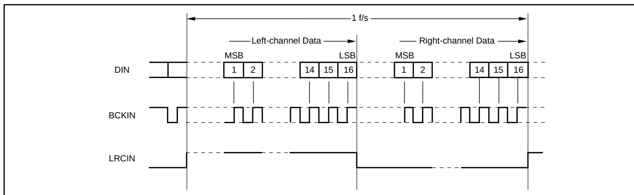
FIGURE 1. Normal Format, 16-Bit (LRCIN H: Lch).
