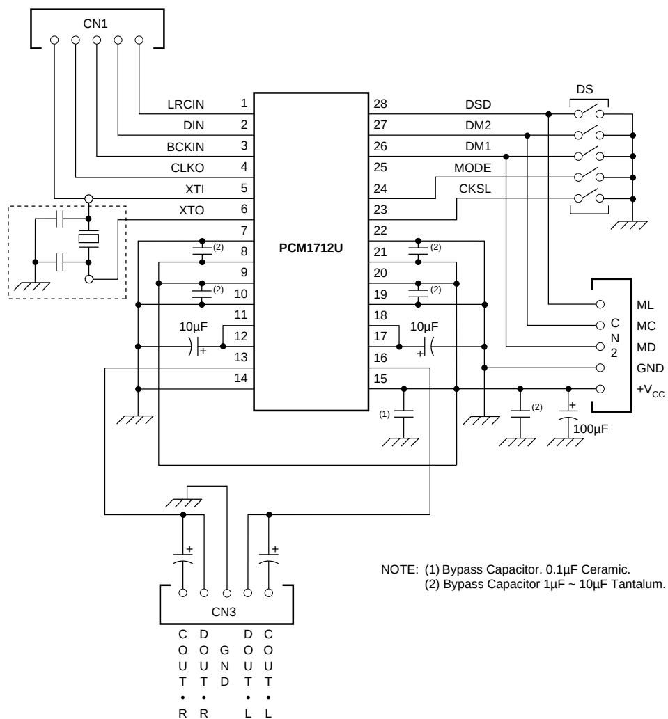
FIGURE 16. DEM-PCM1712 Schematic Circuit Diagram.
