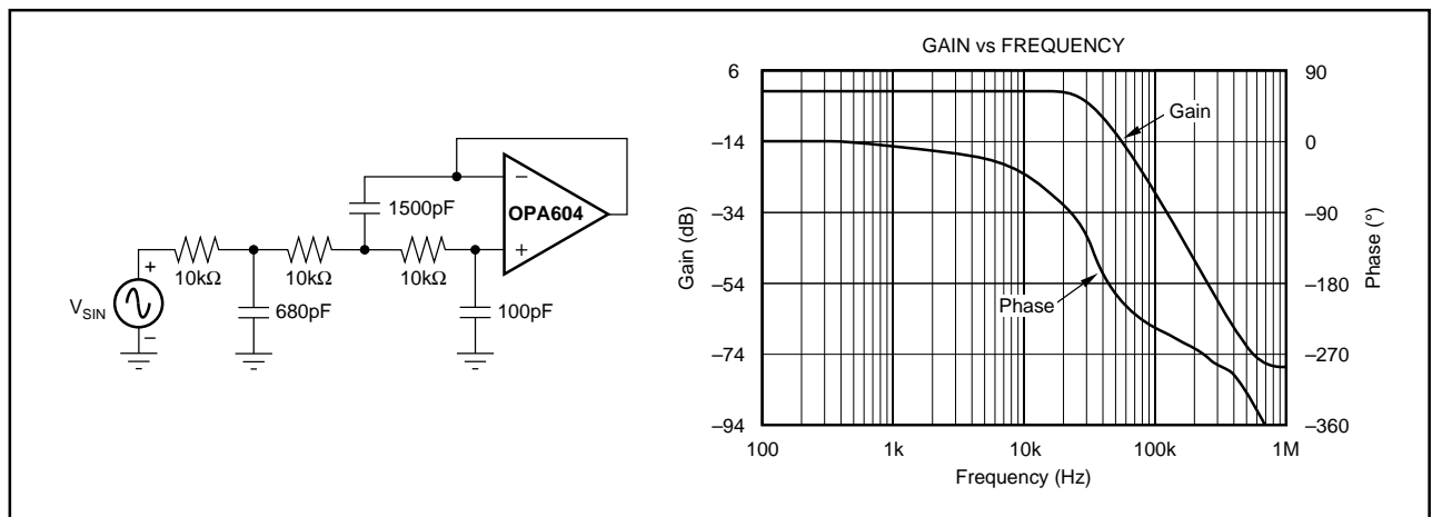
FIGURE 16. 3rd-Order LPF.
