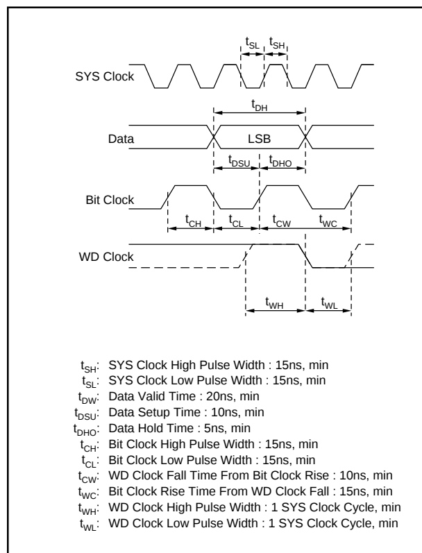
FIGURE 4. Timing Specification.
