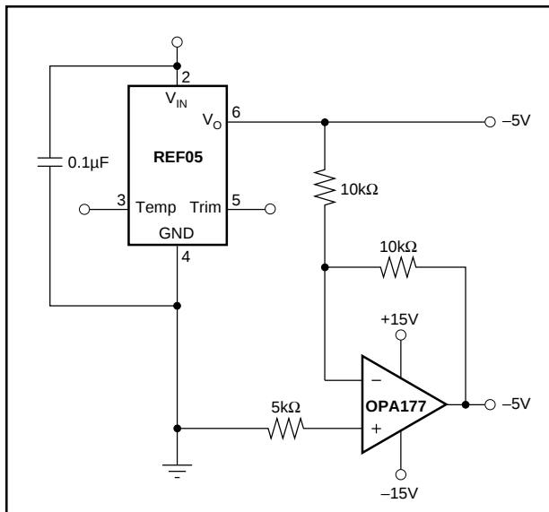
FIGURE 3. \pm 5V Precision Reference.
