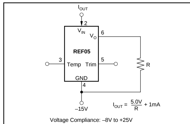
FIGURE 6. Current Sink.
