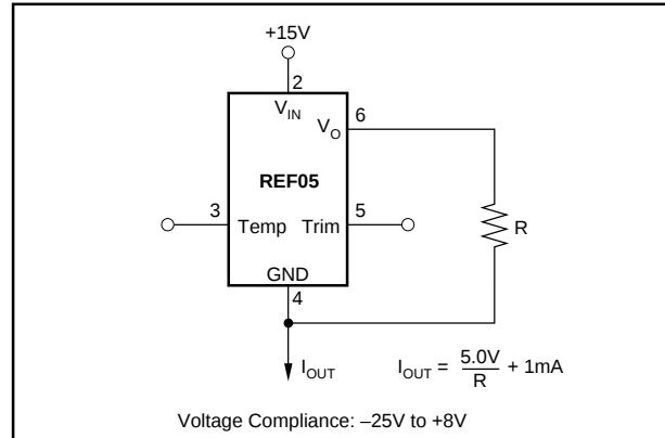
FIGURE 4. Current Source.
