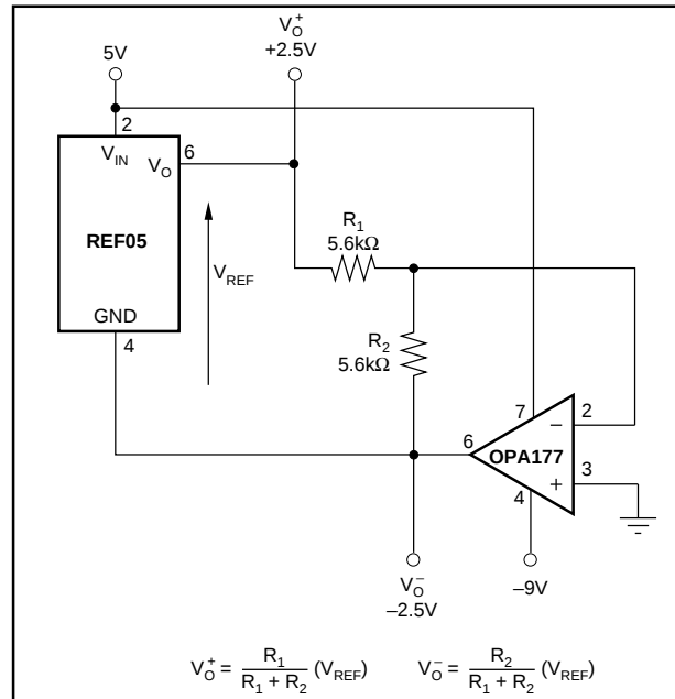
FIGURE 5. \pm 2.5V Precision Reference.
