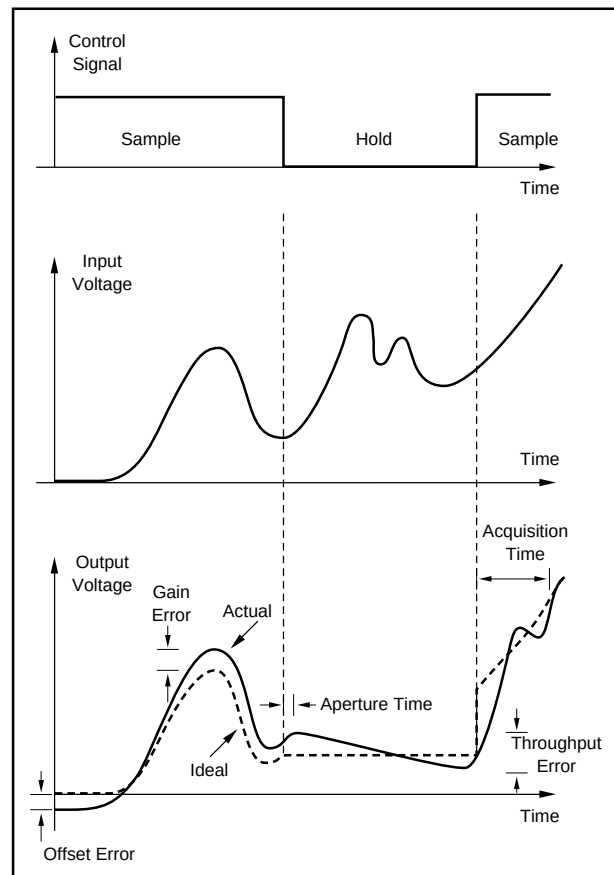
FIGURE 1. Sample/Hold Errors.
