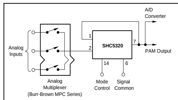
FIGURE 9. Typical Data Acquisition Configuration.
