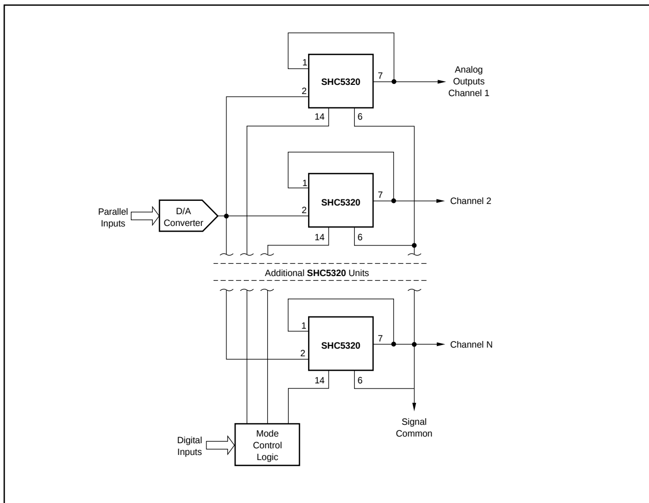
FIGURE 11. Typical Data Distribution Configuration.
