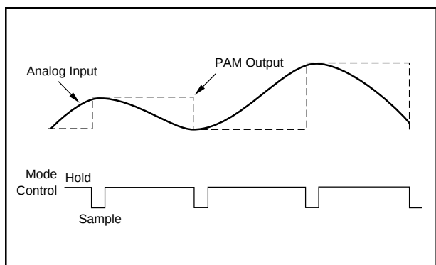
FIGURE 10. PAM Output.
