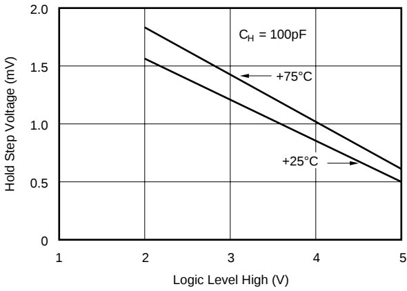
CHARGE OFFSET vs MODE CONTROL ( V_{IH} ) VOLTAGE
