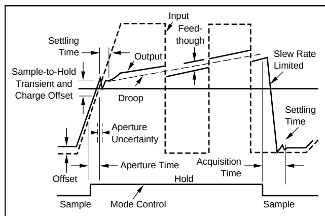
FIGURE 2. Illustration of Sample/Hold Specifications.
