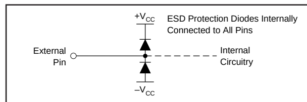
FIGURE 9. Internal ESD Protection.
