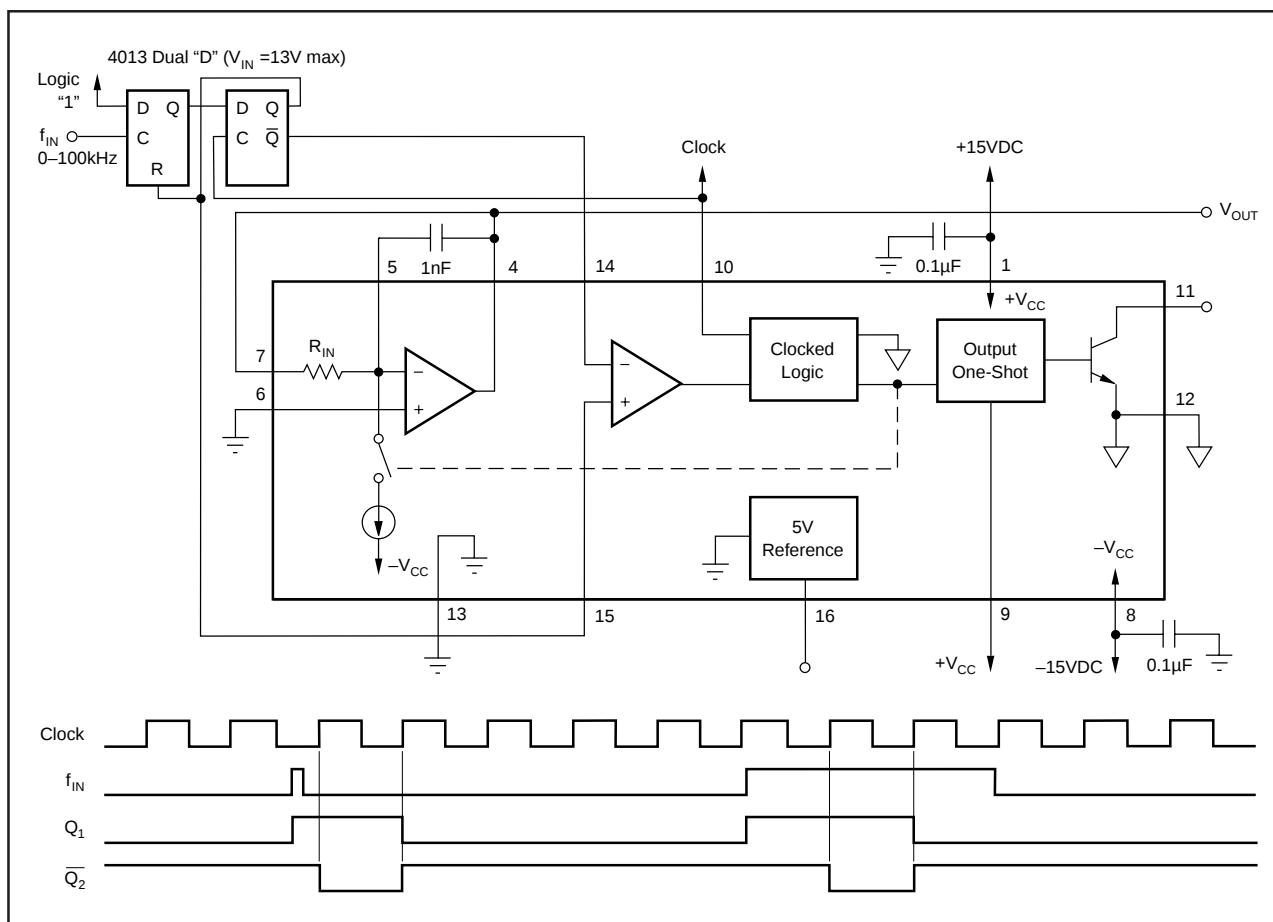
FIGURE 17. Digital Timing Input Conditioning Circuit for Frequency-to-Voltage Operation.
