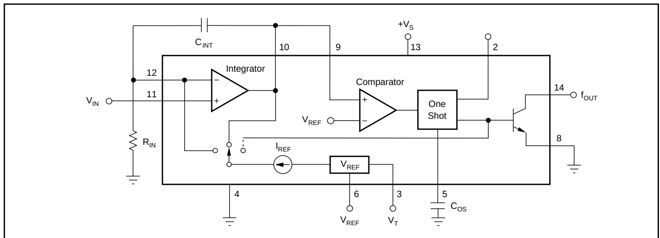
FIGURE 1. VFC121 Architecture.
