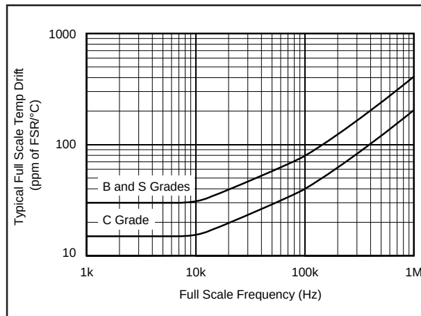
Figure 3. Full Scale Drift vs Full Scale Frequency.
