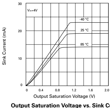
Output Saturation Voltage vs. Sink Current
