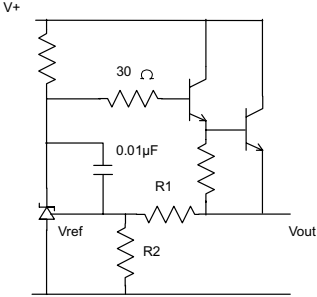
SERIES REGULATOR
