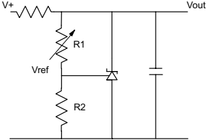
SHUNT REGULATOR
