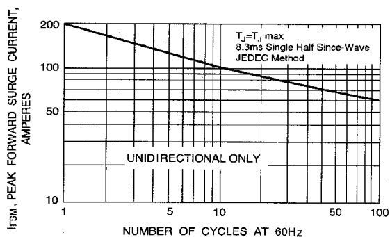
FIG. 6-MAXIMUM NON-REPETITIVE PEAK FORWARD SURGE CURRENT UNIDIRECTIONAL
