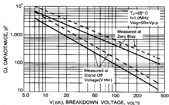
FIG. 4-TYPICAL JUNCTION CAPACITANCE
