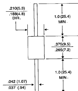
DO-201AE
